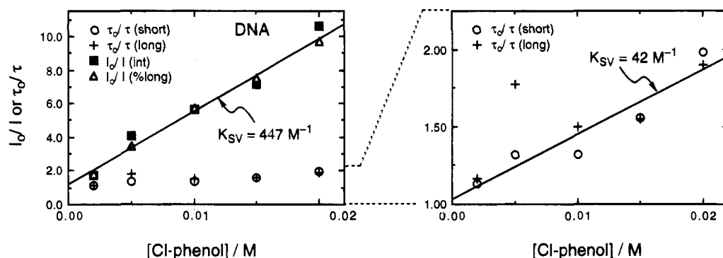
Figure 5. Stern–Volmer plots for the quenching of the short and long lifetime component and the emission intensity of 8 \mu\text{M } ^*\text{Ru}(\text{phen})_2(\text{dppz})^{2+} by o -chlorophenol in the presence of 80 \mu\text{M} calf-thymus DNA (in 5 \text{ mM} Trizma buffer, 50 \text{ mM} NaCl). The left panel shows the difference in the slopes between the intensity (see text) and lifetime quenching, whereas the right panel is an expansion of the left and shows the quenching of both lifetime components.
