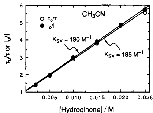
Figure 2. Stern–Volmer plots of the quenching of the emission lifetime and intensity of *Ru(phen) 2 (dppz) 2+ by hydroquinone in acetonitrile.
